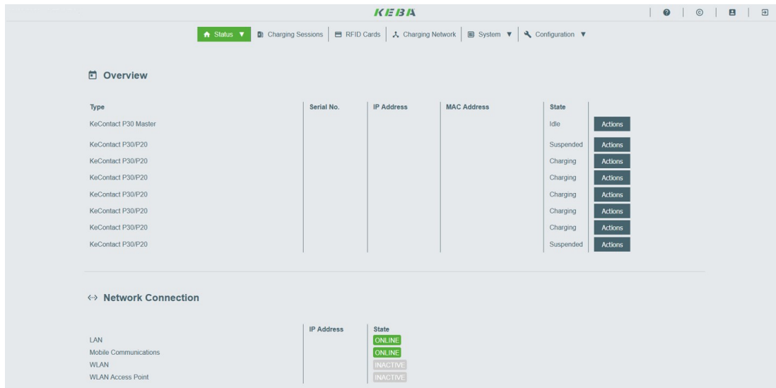
Figure 4. KEBA software
